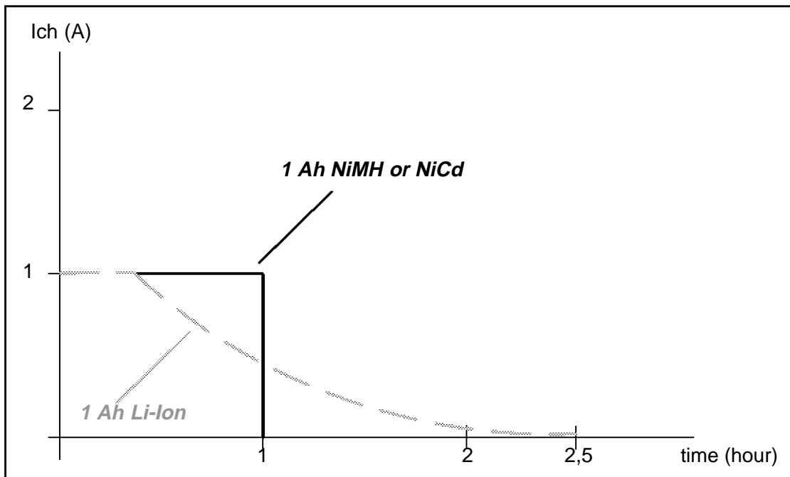
Figure 1-5. A 1 Amp output multicharger will reach full capability of 1Ah pack in: - in 1 hour for NiCd and NiMH batteries - in 2.5 hours for Li-Ion batteries
