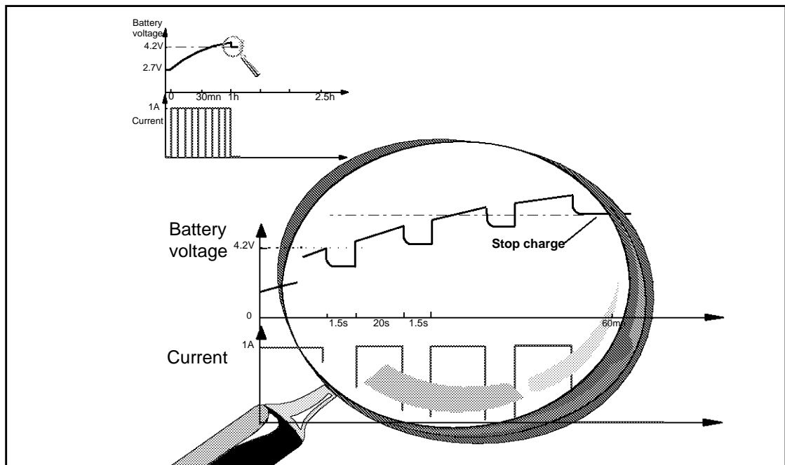
Figure 1-8. To measure “no charge” battery voltage, the charging current delivered by the switching power supply is interrupted by the microcontroller every 20 seconds.
