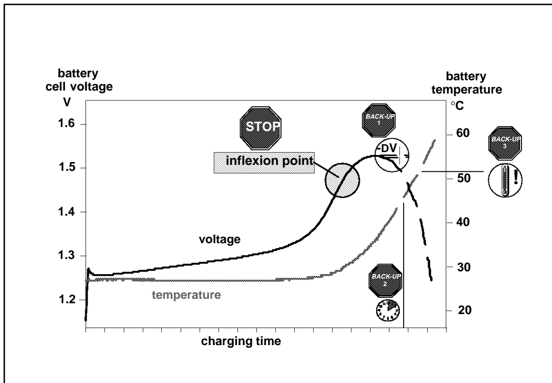
Figure 1-3. Safe charging of NiCd and NiMH batteries is ensured by combining three back-up termination methods: -\Delta V detection, battery temperature monitoring and timed shutdown.
