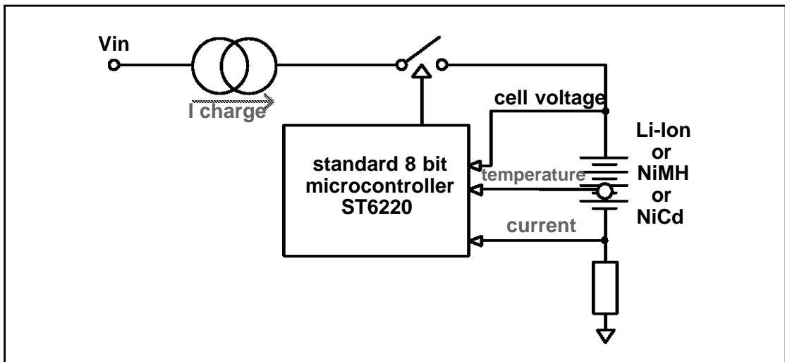
Figure 1-1. Intelligent multicharger concept: Li-Ion/NiCd/NiMH compatibility is ensured by an SGS-THOMSON low-cost 8 bit microcontroller.
