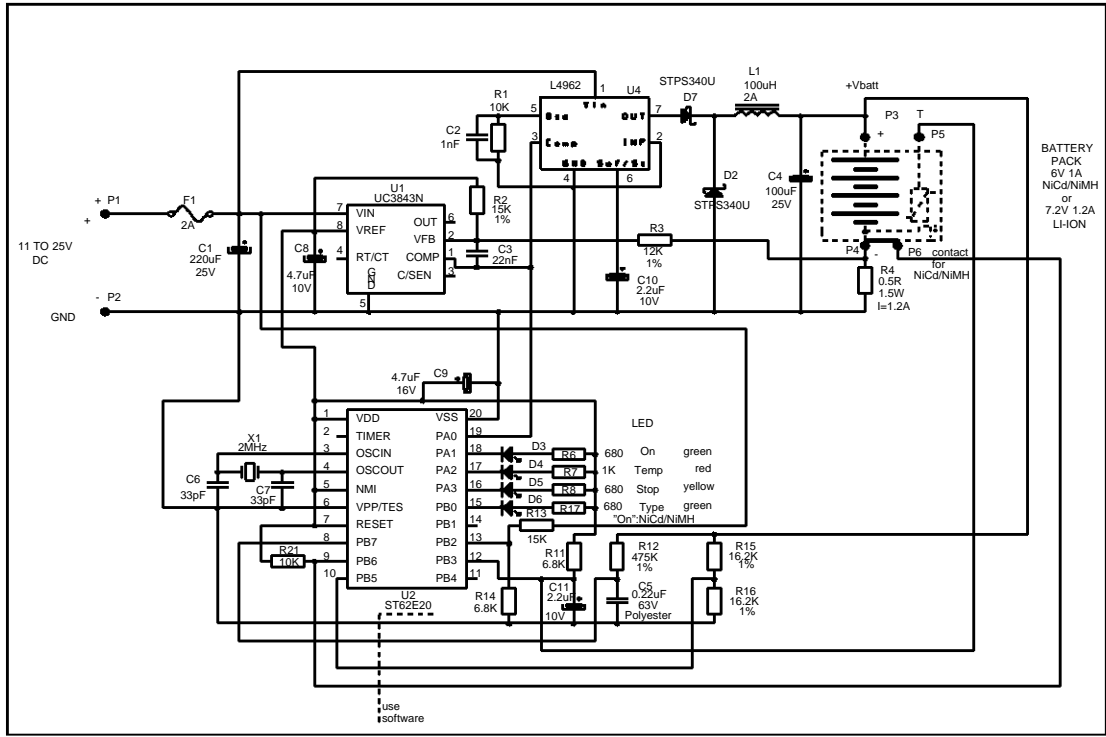
Figure 1-10. Electrical diagram of the Li-Ion/NiCd/NiMH multicharger: DC/DC 100 kHz SMPS/10 Watts
