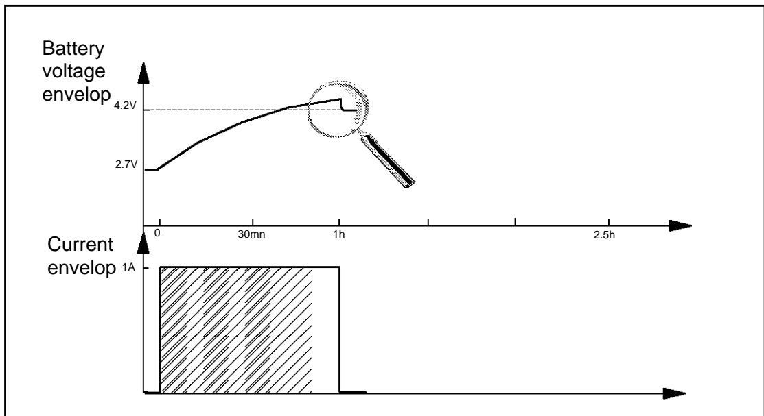
Figure 1-7. New Li-Ion charging method using a constant current source charger: battery voltage and current envelopes
