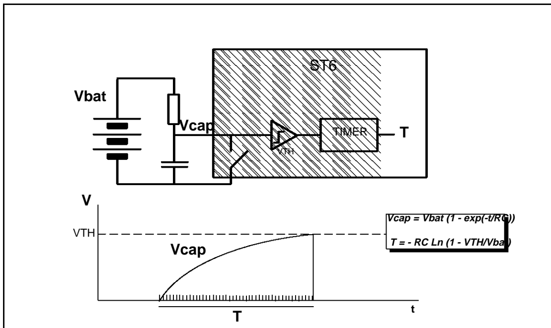
Figure 1-2. RC charge time voltage measurement technique
