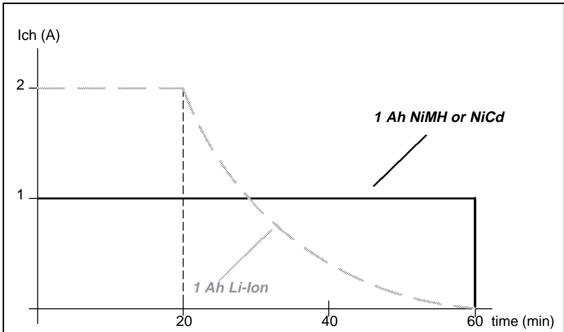
Figure 1-6. To reach full capacity of a 1 Ah Li-Ion pack in one hour, a multicharger must deliver twice the output power with a conventional method, compared to a constant current source method.
